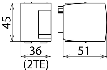
Dimension drawing DR MOD 4P 255
