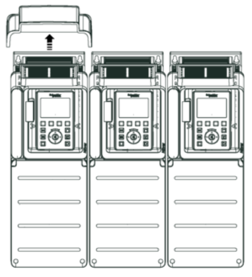
Mounting Type B: Side by Side IP20
