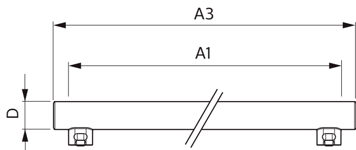
LED 2.2W 300mm S14S WW ND 1CT/4
