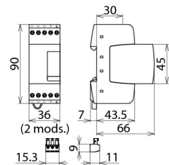
Dimension drawing DR M 4P 255 FM
