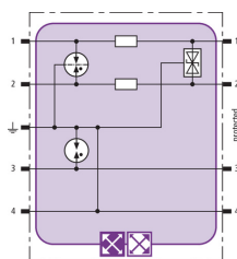
Basic circuit diagram BXT ML2 BE HFS
