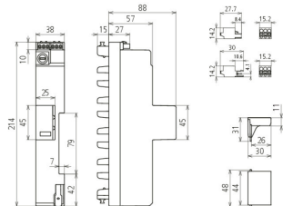
Dimension drawing DSH ZP 2 SG TT 255
