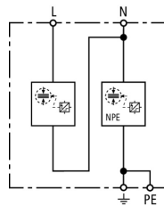
Basic circuit diagram DSH TT 2P 255
