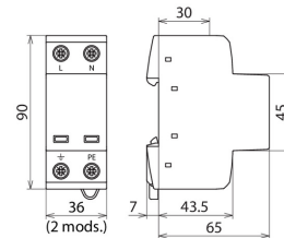
Dimension drawing DSH TT 2P 255
