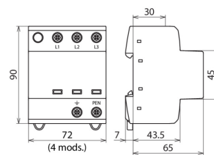
Dimension drawing DSH TNC 255
