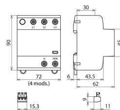
Dimension drawing DSH TNC 255 FM
