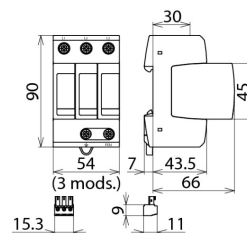
Dimension drawing DG M TNC 440 FM
