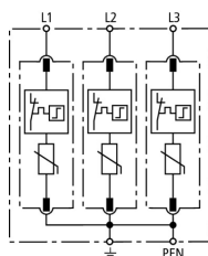
Basic circuit diagram DG M TNC 150
