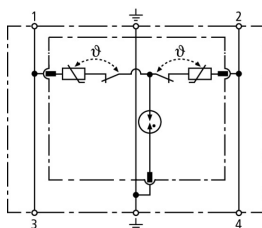
Basic circuit diagram DR M 2P 30
