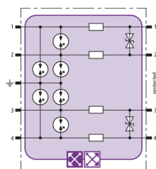
Basic circuit diagram BXT ML4 BD EX 24
