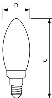
MAS LEDCandleDT5.9-60W E14 927 B35 CL G
