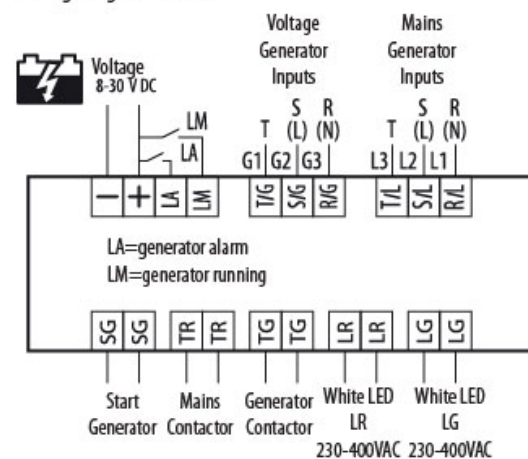
Wiring Diagram ATC-B
