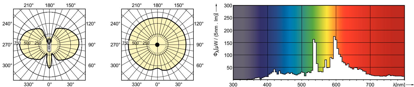
LDLD_CDM-T_70W_830-Light distribution diagram
