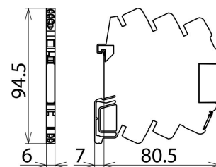
Dimension drawing DCO SD2 MD EX 24
