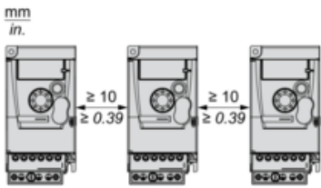
Mounting Type B
