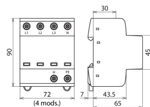
Dimension drawing DSH TT 255
