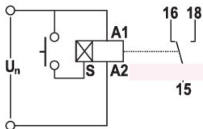
3-wire connection
