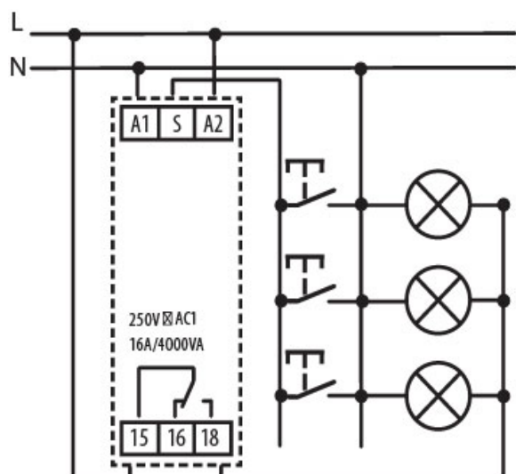
3-wire connection
