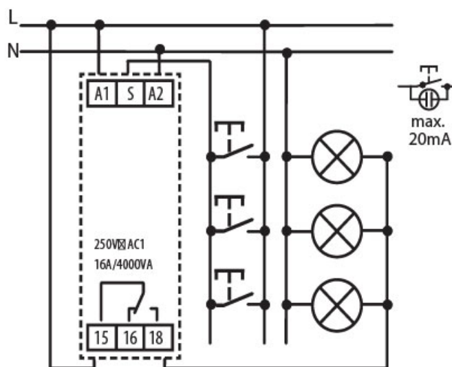
4-wire connection
