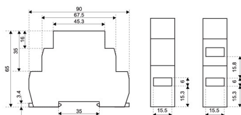
1-module design
