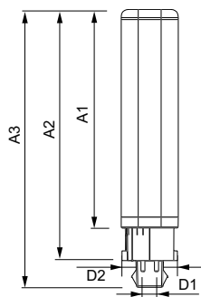
CorePro LED PLC 9W 840 4P G24q-3
